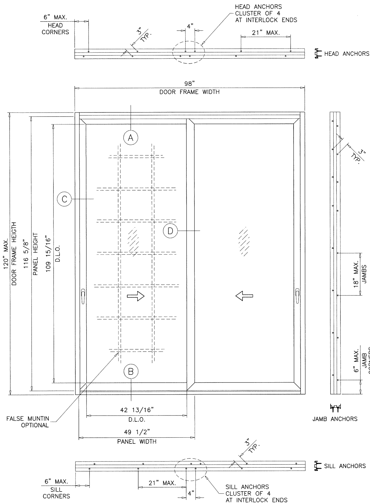
TYPICAL ELEVATION (2 TRACK)
