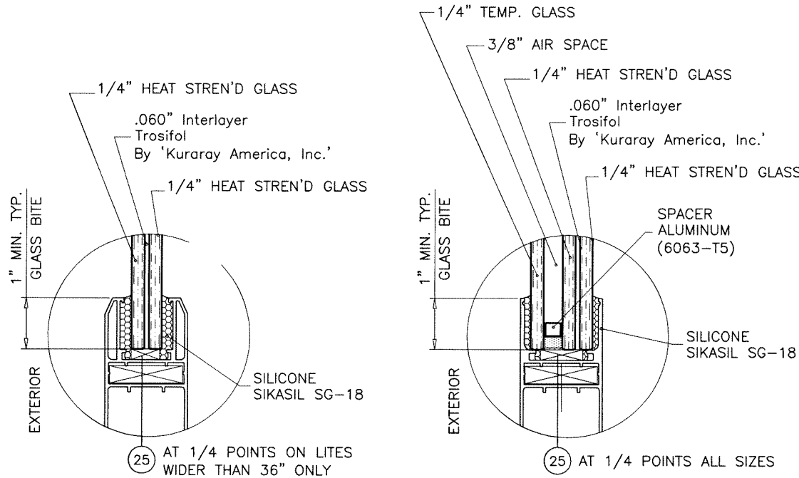
GLASS TYPE 'A' 9/16" OVERALL LAMINATED GLASS
