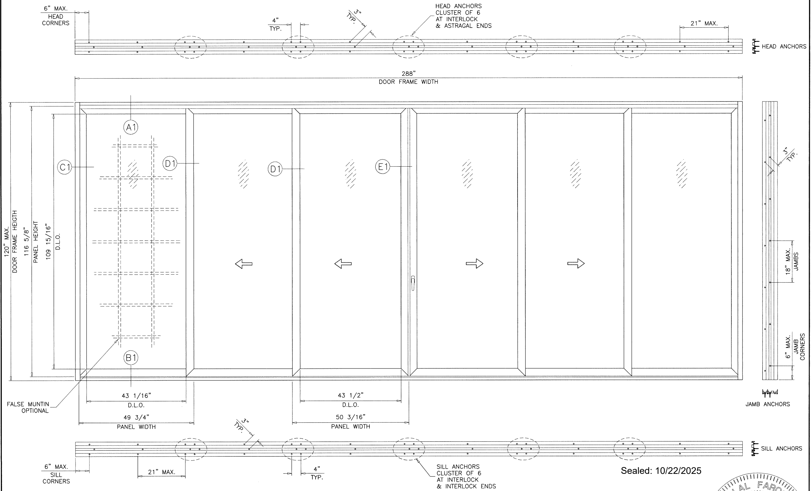
TYPICAL ELEVATION (3 TRACK)
